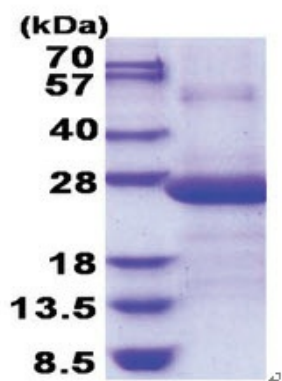
15% SDS-PAGE (3ug)
